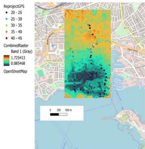
Figure 1 Combined raster image of vegetation and traffic density with NO 2 concentration in Plymouth city centre (9:30-10:30, 20/2/2024). In the raster band, greener colours mean more vegetation and less traffic.
